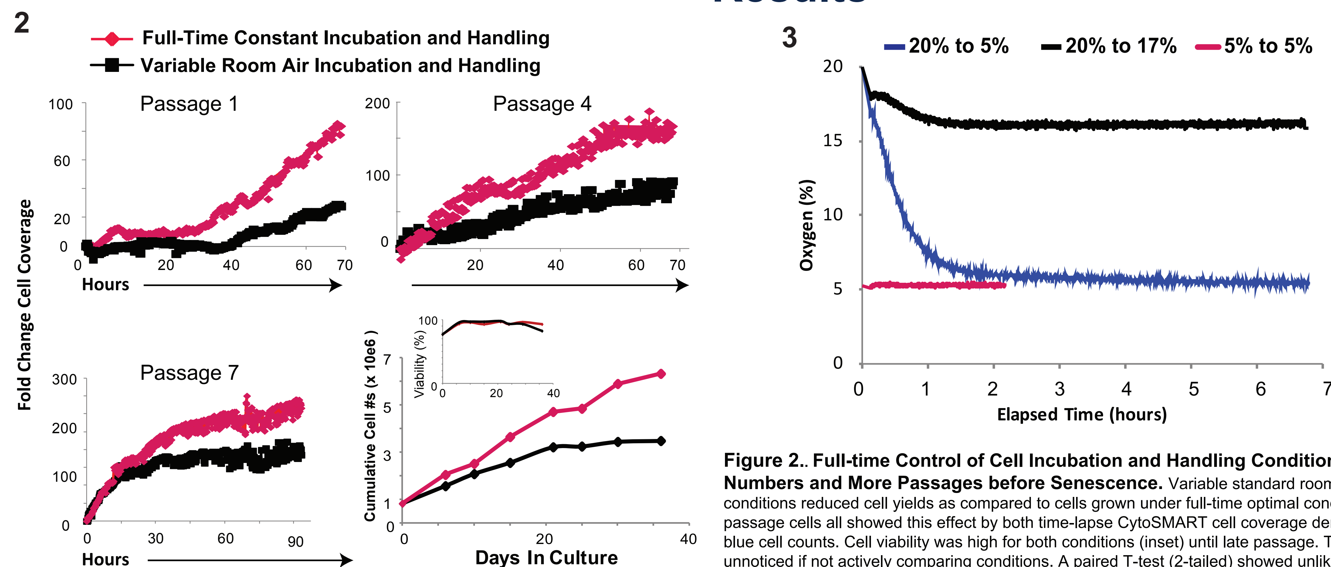
Figure 3. It takes Hours to Equilibrate Medium with Incubator \text{O}_2 . An \text{O}_2 sensor was sealed through the wall of a T-25 flask and \text{O}_2 levels recorded. It took over an hour for medium at room air \text{O}_2 (21%) to equilibrate to the lower room air incubator (17-18%) and almost 7 hrs for medium to equilibrate to physiologic 5% \text{O}_2 . Medium under controlled conditions for cell handling at constant 5% \text{O}_2 and \text{CO}_2 took no time to equilibrate. It only takes 5 min for HIF-1a to be modulated, so hours-long equilibration times may affect cell proliferation and differentiation.
