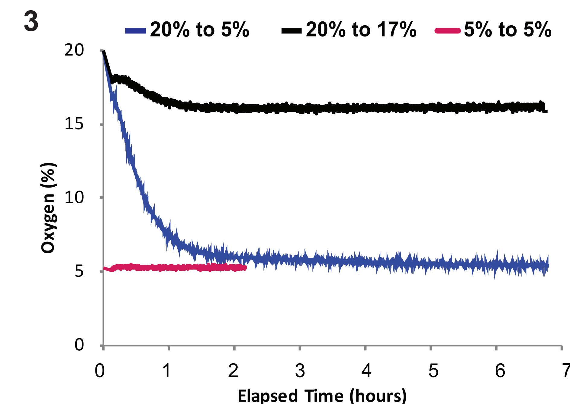
Figure 3. It takes Hours to Equilibrate Medium with Incubator \text{O}_2 . An \text{O}_2 sensor was sealed through the wall of a T-25 flask and \text{O}_2 levels recorded. It took over an hour for medium at room air \text{O}_2 (21%) to equilibrate to the lower room air incubator (17-18%) and almost 7 hrs for medium to equilibrate to physiologic 5% \text{O}_2 . Medium under controlled conditions for cell handling at constant 5% \text{O}_2 and \text{CO}_2 took no time to equilibrate. It only takes 5 min for HIF-1a to be modulated, so hours-long equilibration times may affect cell proliferation and differentiation.
